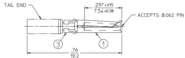
2 PIECE SOCKETS
