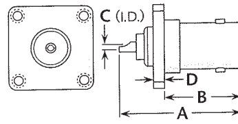
Figure 2 (Solder pot contact)
