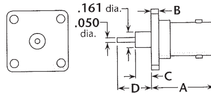
Figure 4 (Post contact)
