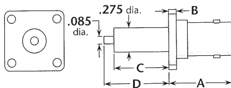
Figure 5 (Post contact)
